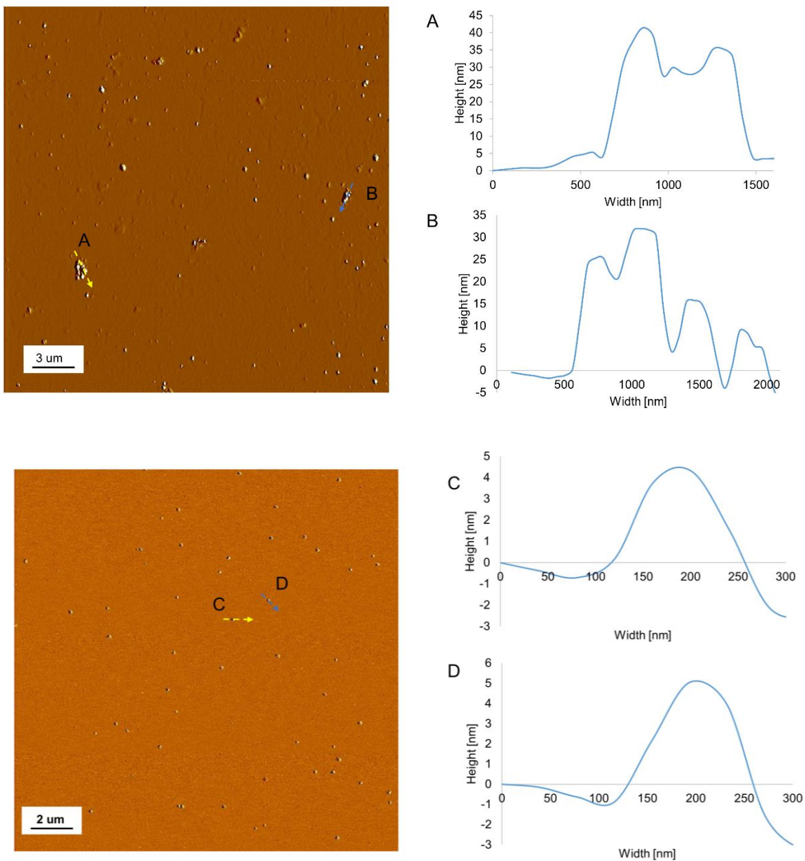
Figure 69. AFM images of the oligomer 1 in the aggregated state (top left) and in the self-assembled state (bottom left). Self-assembly results in spherical nanoparticles. Self-assembly was performed with slow cooling (1°C/min) from 70 °C to 20 °C. Conditions: oligomer 1 (1 μM), 10 mM sodium phosphate buffer, pH 7.2, 20 vol% EtOH.
