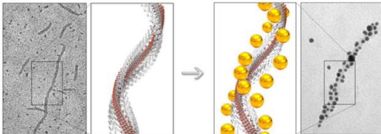
Figure 55. Functionalization of the DNA-grafted SPs with AuNPs. Taken from [22].
