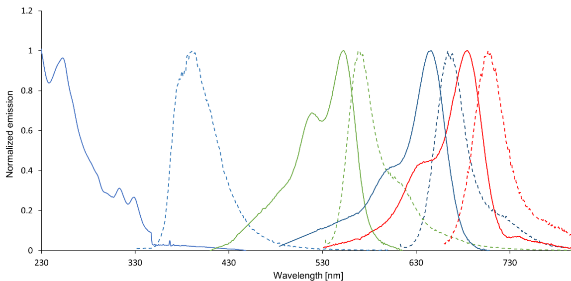
Figure 16: Normalized spectral overlap. Absorption (solid line) and emission (dotted line) spectra for LHCs: SPs (blue), Cy3 (green), Cy5 (blue) and Cy5,5 (red).
