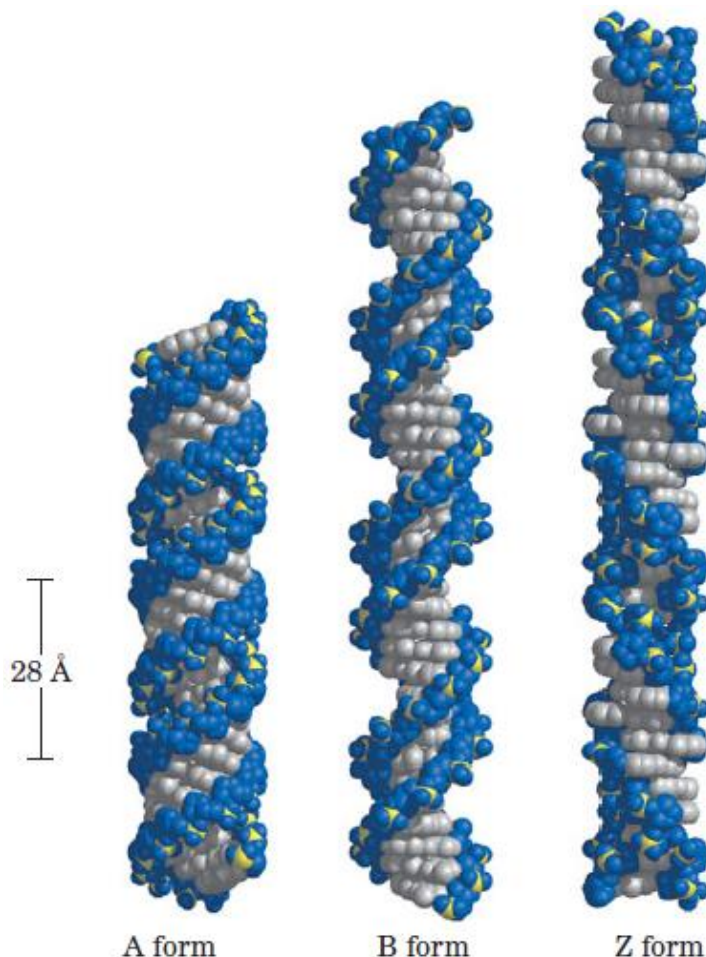
Figure 5. Structural variants of DNA (A, B and Z conformation). [12]
