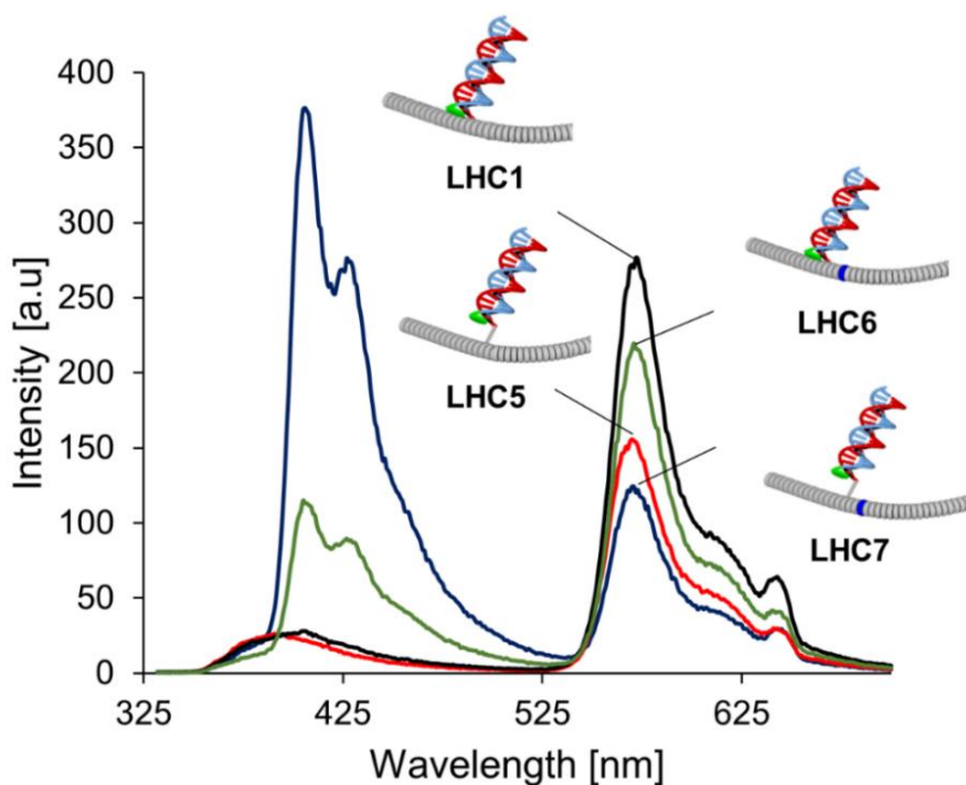
Figure 42. Fluorescence emission spectra of LHC1 (black), LHC5 (red), LHC6 (blue) and LHC7 (green). Concentration of oligomers: A (0.5 \mu M) and 15 nM B , L , M , N and H ; Conditions: 10 mM sodium phosphate buffer, pH 7.2, 120 mM NaCl, \lambda_{\text{ex}} : 322 nm.
