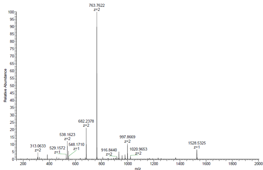
Figure 71. ESI-MS analysis of oligomer 1.
