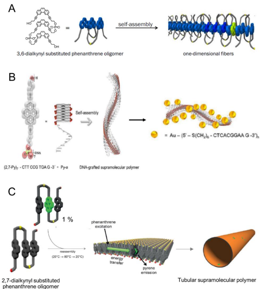
Figure 13. Previously investigated oligomers which self-assemble in aqueous medium. A) 3,6-Dialkynyl phenanthrene; [70] B) 2,7-Dialkynyl pyrene DNA conjugate and DNA-grafted supramolecular polymers functionalized with AuNPs; [22] C) 2,7-dialkynyl phenanthrene; [61] the nanotubes and the fibers act as light-harvesting antenna with an incorporated acceptor (pyrene is highlighted in green).
