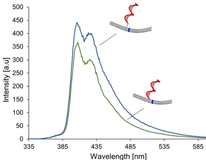
Figure 36. Fluorescence spectra of self-assembled SPs composed of oligomer A (0.5 \mu\text{M} ) and either oligomer N (15nM) or oligomer M (15nM) in sodium phosphate buffer, pH 7.2, 120 mM NaCl, \lambda_{\text{ex}} : 322 nm.
