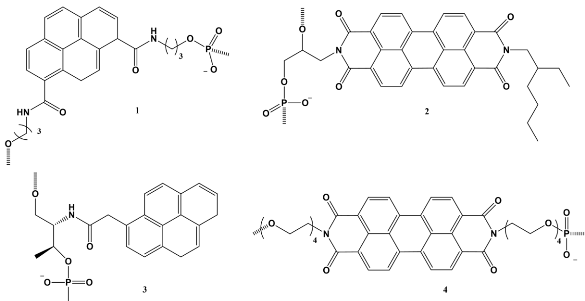
Figure 7. Different ways to link non-nucleosidic chromophores, such as pyrene or perylenebisimide, with DNA backbone via acyclic linker, 1: carboxamide-linker, [24] 2: (S)-aminopropan-2,3-diol linker, [26] 3: threoninol linker, [32] 4: tetraethylene glycol-linker. [27]
