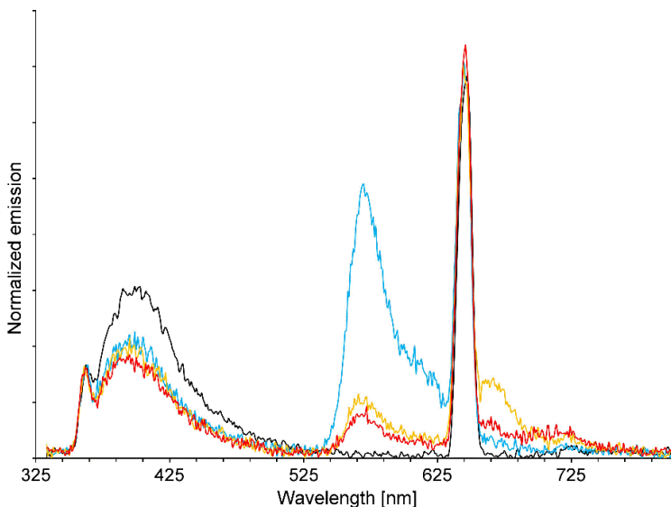
Figure 23. Fluorescence emission spectra of LHC1 (green), LHC2 (orange), LHC3 (red) and LHC4 (black). Concentration of oligomers: A (0.5 \mu\text{M} ), B , C , D , E , F and H (15 nM). Concentration of oligomers: A (0.5 \mu\text{M} ), B , C , D , E , F and H (15 nM). Conditions: 10 mM sodium phosphate buffer, pH 7.2, 120 mM NaCl, \lambda_{\text{ex}} = 322 nm.
