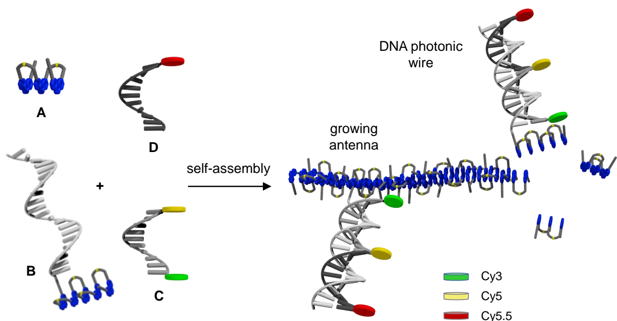
Figure 14. Illustration of the supramolecular assembly of a light-harvesting complex (LHC3). Chromophore-modified DNA hybrids containing terminal phenanthrenes (shown in blue) are incorporated into the growing phenanthrene antenna during supramolecular polymerization.
