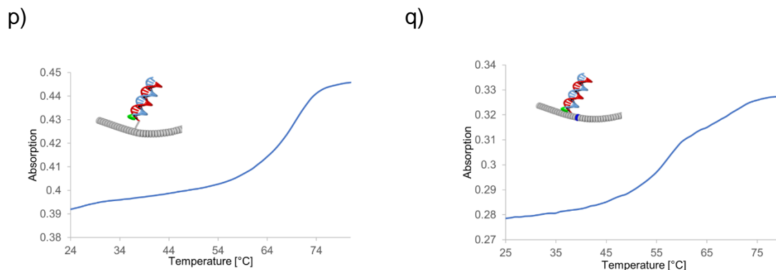
Figure 54. Melting curves of complexes: l) A and N ; m) A and L ; n) A and M ; o) A , N and H ; p) A , L and H ; q) A , M and H ; Condition: see Table 11.3.3 Integration of DNA-Modified Gold Nanoparticles into Supramolecular Polymers
