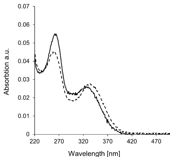
Figure 66. UV-Vis spectra of the aggregated (20 °C, dashed) and disassembled (70 °C, solid curve) state. Concentration of oligomer 1 : 1 \mu M, 10mM sodium phosphate buffer pH 7.2, 20 vol% EtOH.
