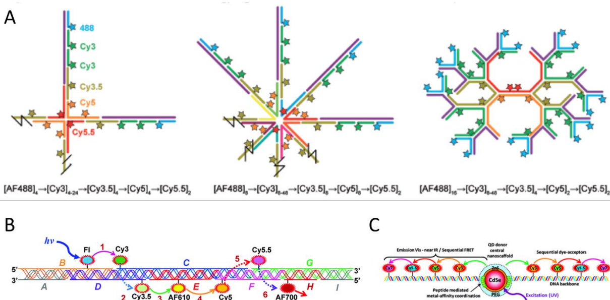
Figure 11. Examples of photonic wires designed in Medintz group. A: Four arm, eight-arm, and 2:1 dendrimeric DNA photonic wires with extended homo FRET. B: Linear DNA photonic wires with 7 fluorophores arranged along the DNA scaffold. C: DNA photonic wires that self-assemble around the quantum-dot.
