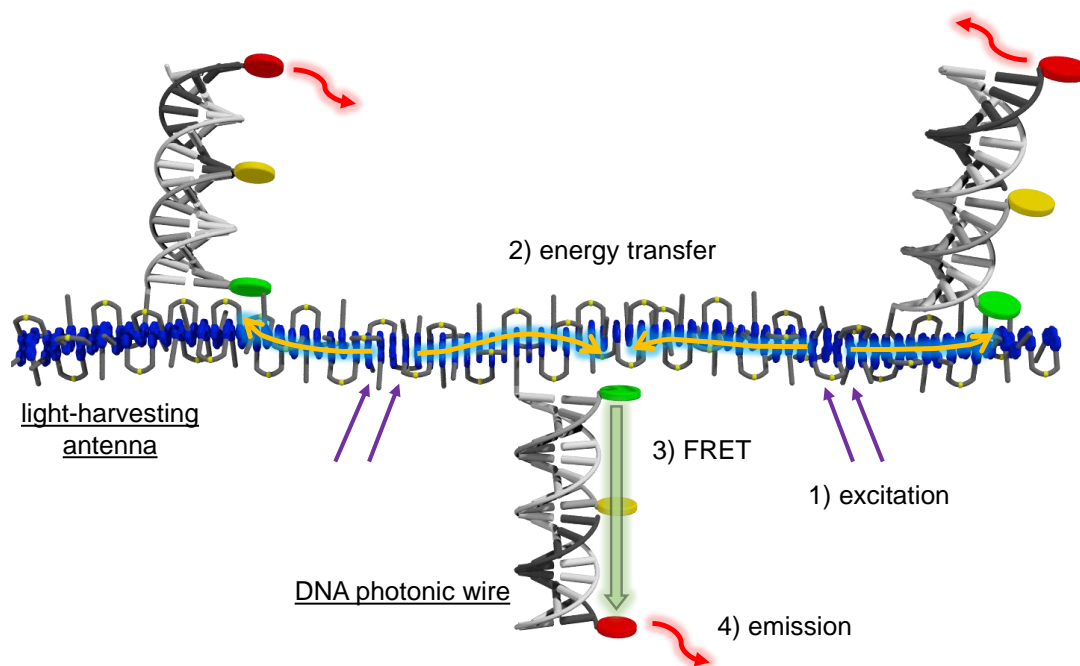
Figure 17. Illustration of light-harvesting complex LHC3 : DNA photonic wires bearing suitable acceptor dyes (Cy3, Cy5 and Cy5.5 in green, yellow and red) are integrated into a supramolecular polymer ('antenna') composed of phenanthrenes (blue). Excitation energy absorbed by phenanthrene molecules is transferred along the antenna to the acceptor dye (Cy3) and further along the DNA photonic wire via FRET.
