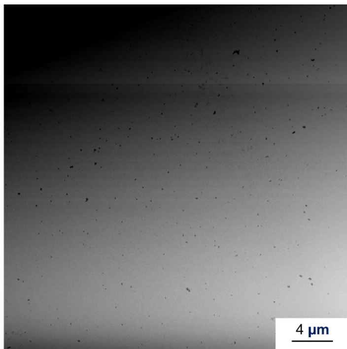
Figure 59. AFM image of the Au-NP modified DNA. Conditions: T (150 nM) in 10 mM sodium phosphate buffer, pH 7.2, 120 mM NaCl.
