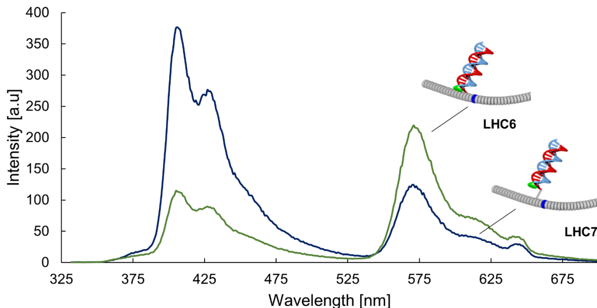
Figure 39. Fluorescence emission spectra of LHC6 (blue) and LHC7 (green). Conditions: concentration of oligomers: A (0.5 \mu M), N, M, H (15 nM); 10 mM sodium phosphate buffer, pH 7.2, 120 mM NaCl, \lambda_{\text{ex}} : 322 nm.
