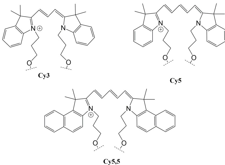
Figure 32. Structures of the non-nucleosidic building blocks (donors – acceptors) in DNA photonic wire.
