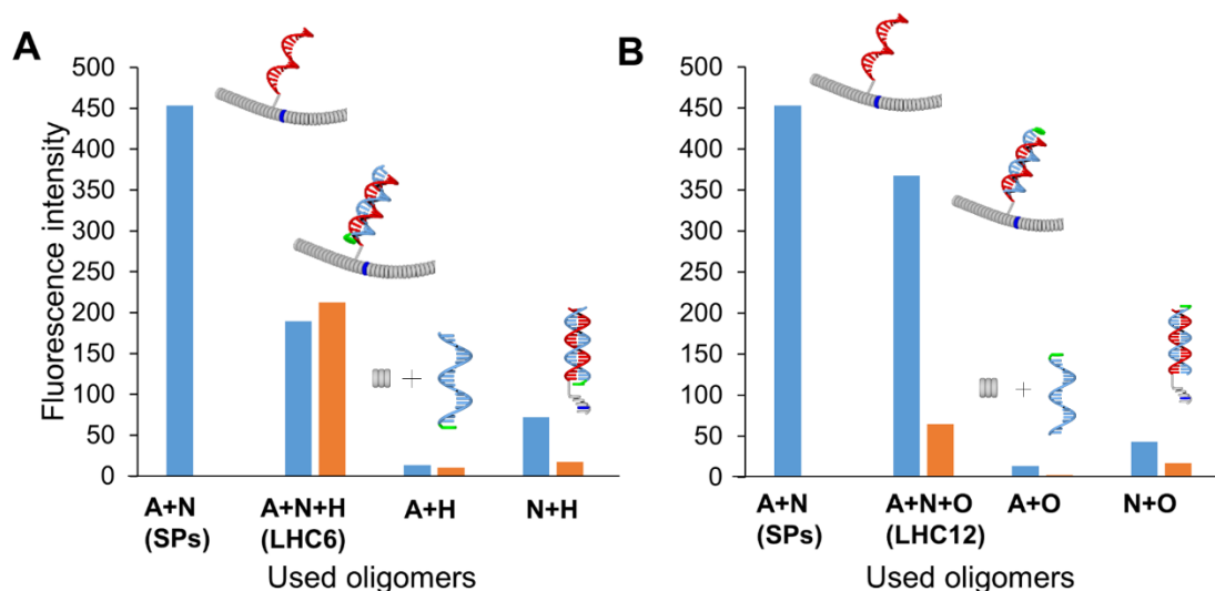
Figure 45. Diagram with the integrated fluorescence emission spectra of SPs alone (oligomer A , N ) LHC6 (A) or LHC12 (B) as well as a mixture of either oligomer A or N in combination with the Cy3-derived oligonucleotide H (A) or O (B). Integrated fluorescence emission of phenanthrene/pyrene fluorescence / between 335 nm and 520 nm; blue bars) and Cy3 (between 525 nm and 630 nm; orange bars).
