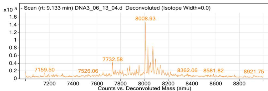
Figure 48. MS analysis of oligomer M.
