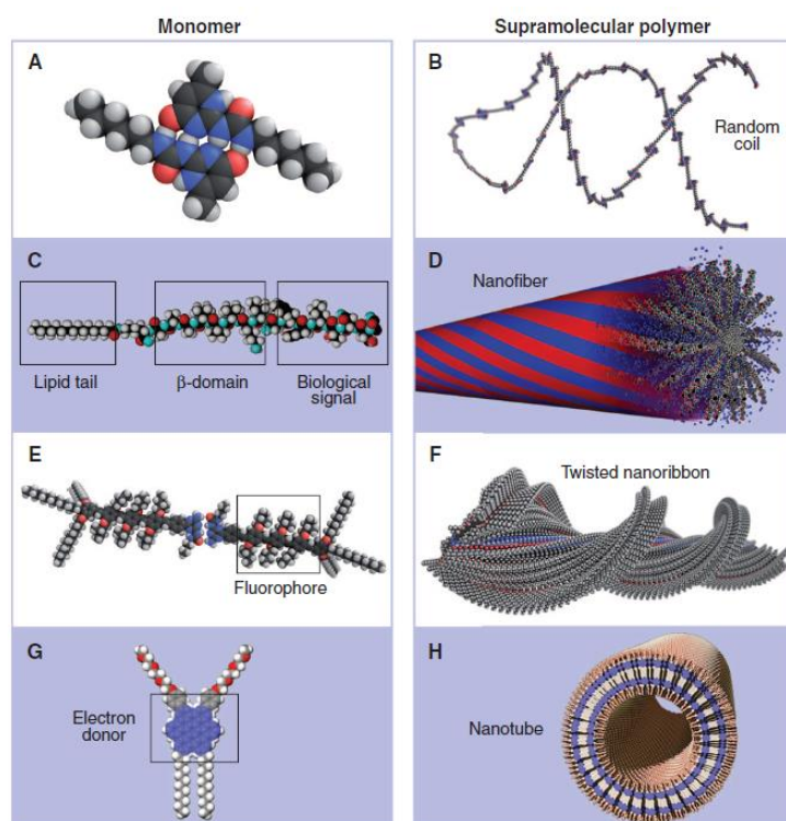
Figure 1. Representation of four different monomeric building blocks and the corresponding supramolecular assemblies with mechanical (A and B), biological (C and D), optical (E and F) or electronic (G and H) functionalities. [3]
