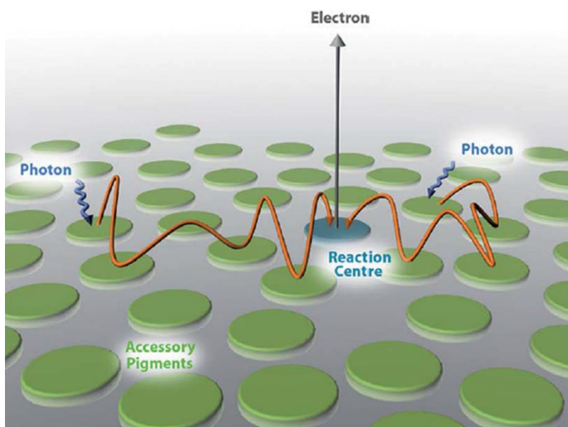
Figure 9. Demonstration of the light-harvesting antenna effect. Photons are captured by light-harvesting pigments and transferred to the reaction centre (the acceptor). In the reaction centre the charge separation occurs and the storage of chemical energy takes place. [37] Taken from [39] .
