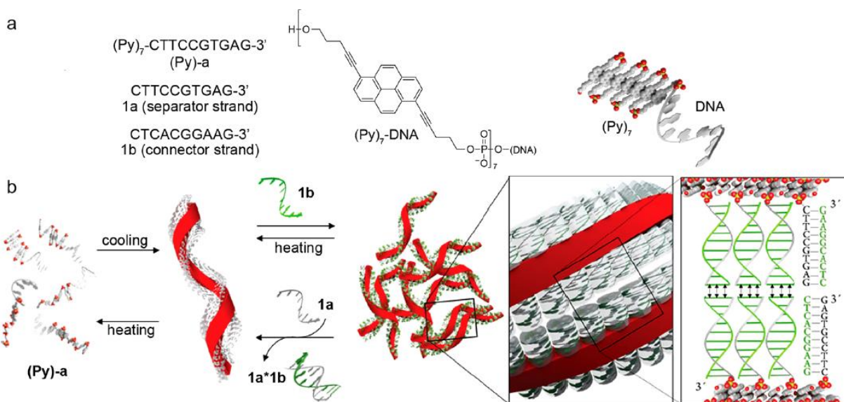
Figure 3. Assembly and disassembly of the nanoribbons composed of chimeric oligomers. Hybridization of the complementary oligonucleotide on the pyrene-modified oligonucleotide leads to the formation of networks via cooperative blunt end. [8]
