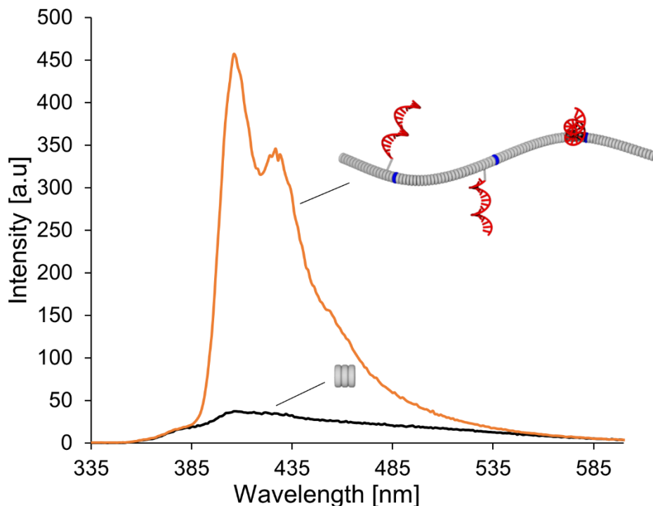
Figure 35. Fluorescence spectra of oligomer A (0.5 \mu\text{M} , black) and self-assembled SPs composed of oligomer A (0.5 \mu\text{M} ) and oligomer N (15nM) in 10 mM sodium phosphate buffer, pH 7.2, 120 mM NaCl, \lambda_{\text{ex}} : 322 nm.
