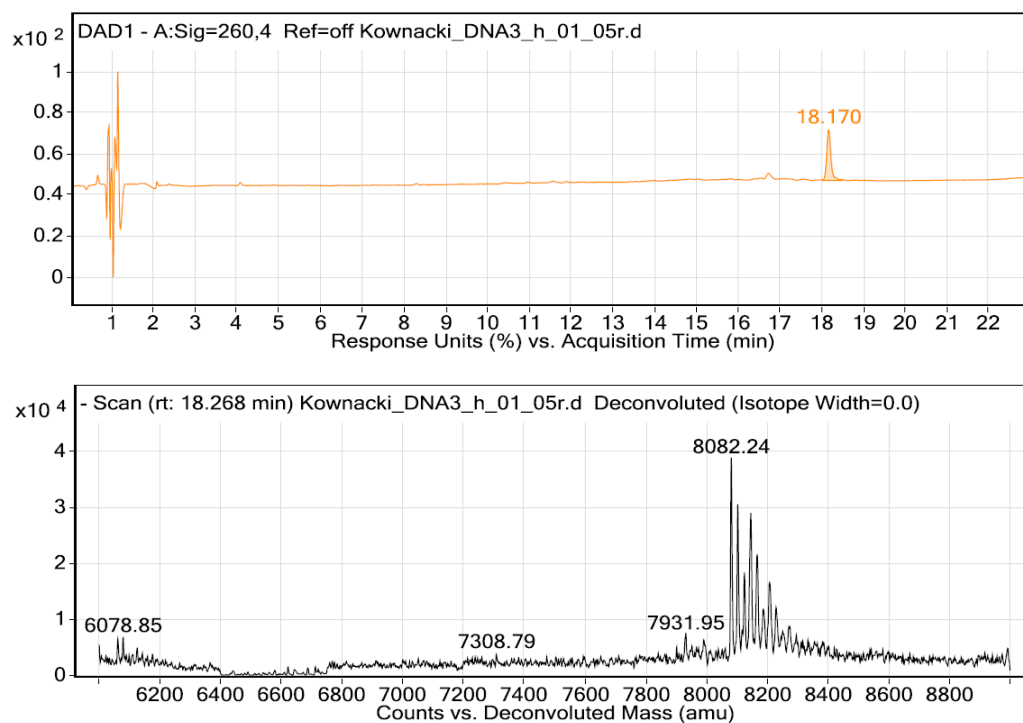
Figure 28. LC-MS analysis of oligomer B.
