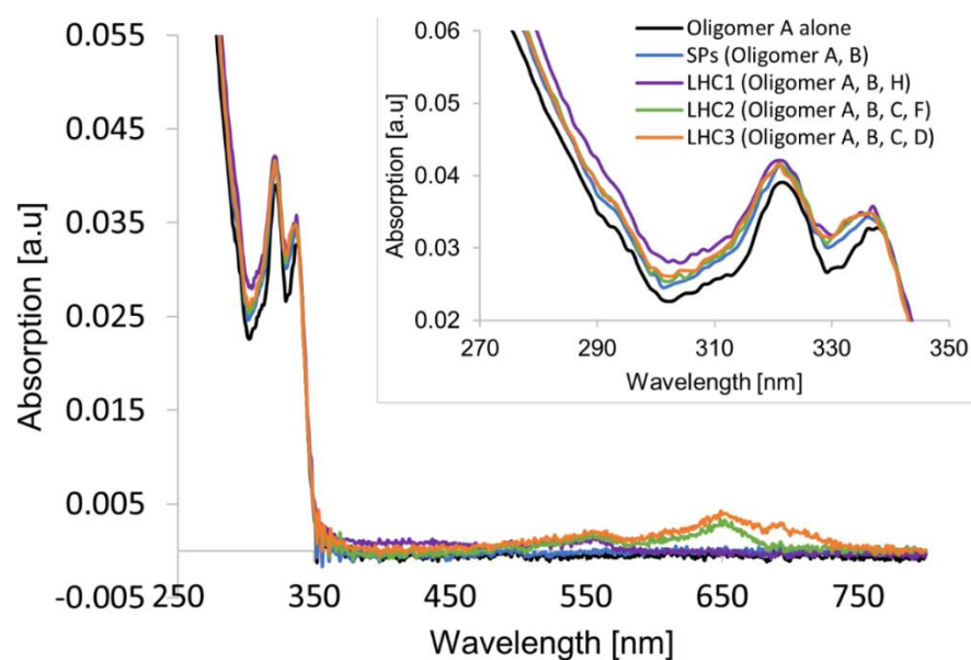
Figure 30. Absorption spectra of oligomer A alone, SPs (oligomer A + B ), LHC1 , LHC2 and LHC3 (0.5 \mu\text{M} oligomer A , 0.015 \mu\text{M} oligomer B , C , D , F , H ). Insert: Enlargement of region 270-350 nm from spectra shown in a). Conditions: 10 mM sodium phosphate buffer, pH 7.2, 120 mM of NaCl.
