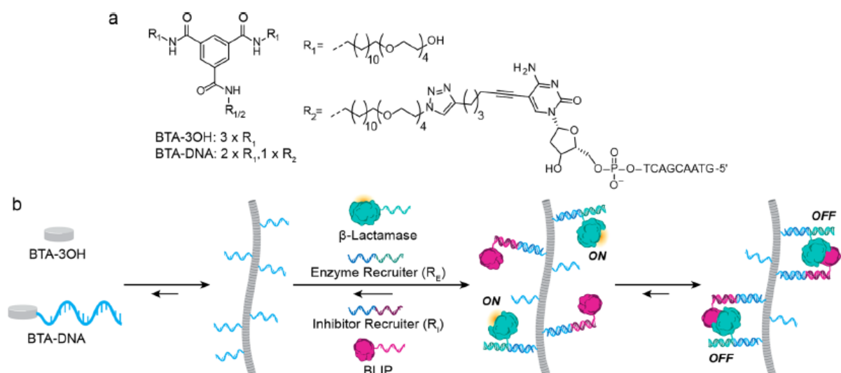
Figure 4. Supramolecular BTA platform used for the recruitment of \beta -lactamase and BLIP. A: Chemical structures of a BTA monomeric building blocks BTA-3OH and BTA-DNA modified with 10 nucleobases. B: Co-assembly of inert BTA and BTA-DNA monomers into DNA-functionalized supramolecular polymers. Selective hybridization of a DNA-modified proteins with the complementary DNA of functionalized polymers is allowed in the presence of a recruiter strand. [9]
