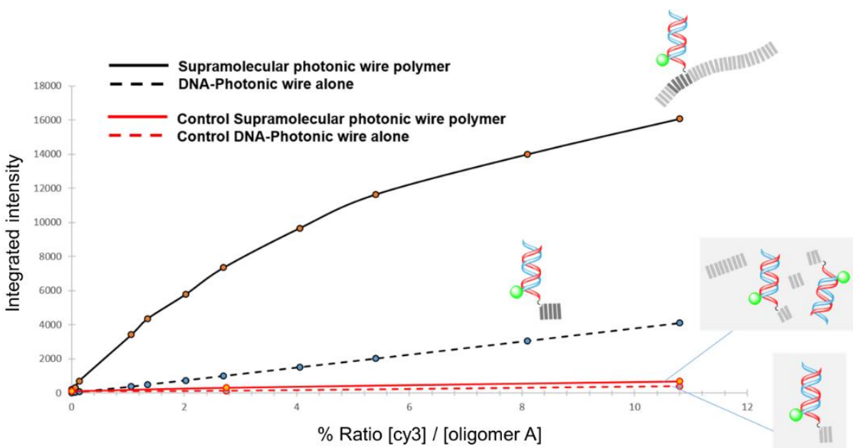
Figure 22. Fluorescence emission titration experiment of oligomers B (black curves) and K (red curves) in the presence of SP formed of oligomer A (note: oligomer K contains only three phenanthrenes and is not integrated into SPs). Fluorescence emission was integrated: 535 - 635 nm.
