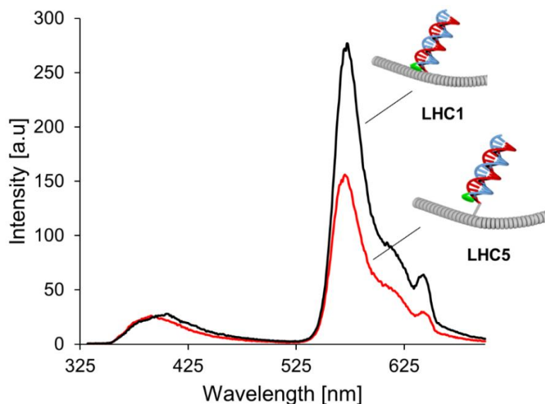
Figure 40. Fluorescence emission spectra of LHC1 (black) and LHC5 (red). Concentration of oligomers: A (0.5 \mu\text{M} ), B , L , H (15 nM); Conditions: 10 mM sodium phosphate buffer, pH 7.2, 120 mM NaCl, \lambda_{\text{ex}} : 322 nm.
