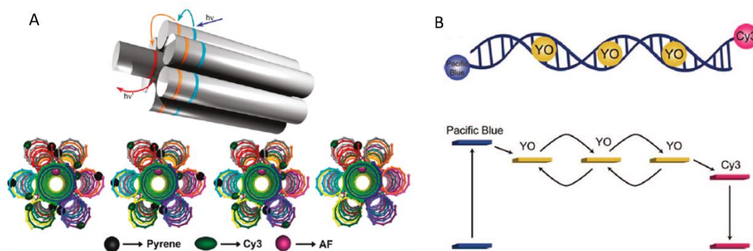
Figure 12. A. Liu's triads for precisely organized donor-acceptor arrays. [45] B. Self-assembled DNA based photonic wire and the energy level diagram with a diffusive energy transfer mechanism proposed by Albinsson. [42]
