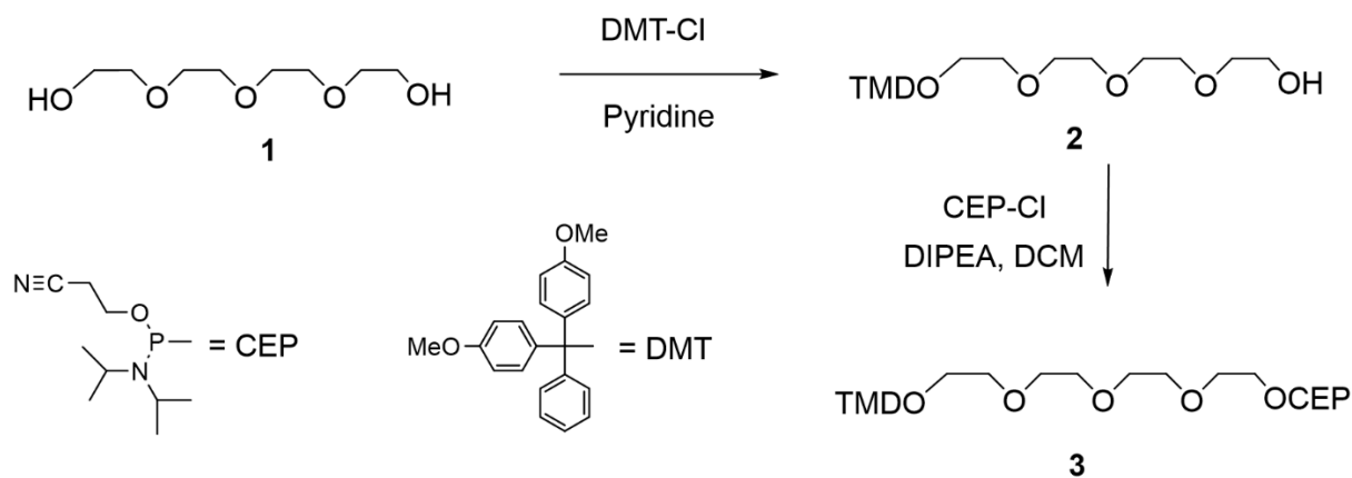
Figure 50. Synthesis of the PEG linker building block.
