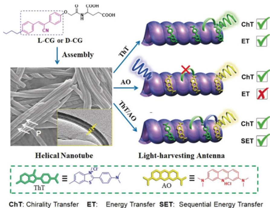
Figure 10. Co-assembly of the supramolecular light harvesting nanotube composed of cyanostilbene-appended glutamate compound (CG) with acceptors (ThT, AO) results in three different chirality and energy transfer patterns. Taken from [41] .
