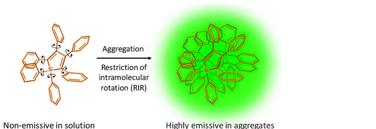
Figure 61. Illustration of AIE-active hexaphenylsilole. Taken from [108]
