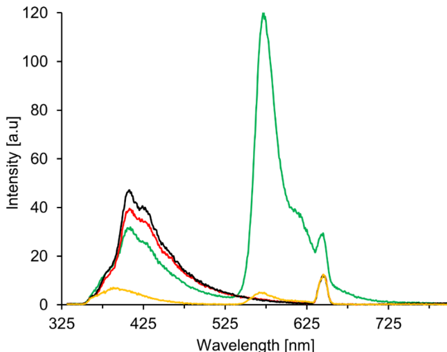
Figure 18. Fluorescence intensities of LHC1 (green), LHC4 (black) or a mixture of either oligomer A (red) or B (light brown) in combination with the Cy3-derived oligonucleotide H . Concentration of oligomers: A (0.5 \mu M), B and H (15 nM); conditions: 10 mM sodium phosphate buffer, pH 7.2, 120 mM NaCl, \lambda_{\text{ex}} = 322 nm.
