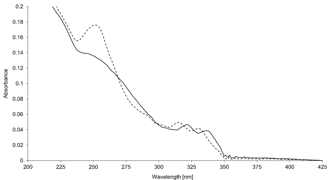
Figure 37. UV-vis spectrum of SPs (oligomer A (0.5 \mu M) and oligomer N (15nM)) in assembled (20 °C, solid curve) and the disassembled state (80 °C, dashed curve) in 10 mM sodium phosphate buffer, pH 7.2, 120 mM NaCl, \lambda_{\text{ex}} : 322 nm.
