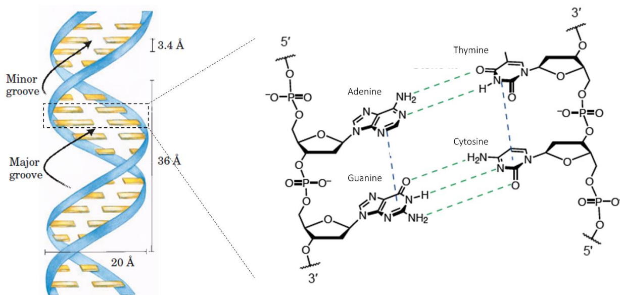
Figure 6. Left: schematic illustration of DNA double helix. Right: Watson – Crick base pairs: adenine (A), guanine (G), thymine (T) and cytosine (C). [12]
