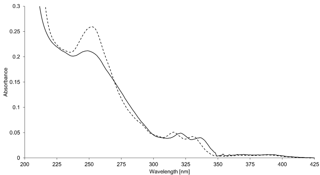
Figure 38. UV-vis spectrum of SPs (oligomer A (0.5 \mu M) and oligomer M (15nM)) in the assembled (20 °C, solid curve) and the disassembled state (80 °C, dashed curve) in 10 mM sodium phosphate buffer, pH 7.2, 120 mM NaCl, \lambda_{\text{ex}} : 322 nm.
