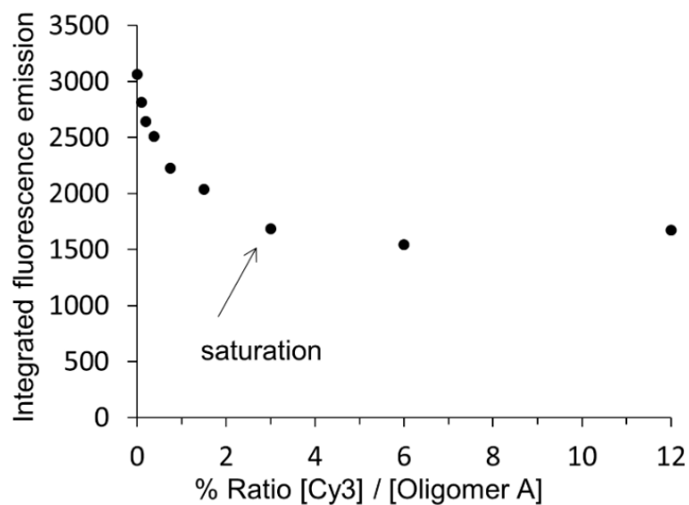
Figure 21. Indication that the SPs are saturated. Change of integrated fluorescence (340-525 nm) after correction for B*G contribution.
