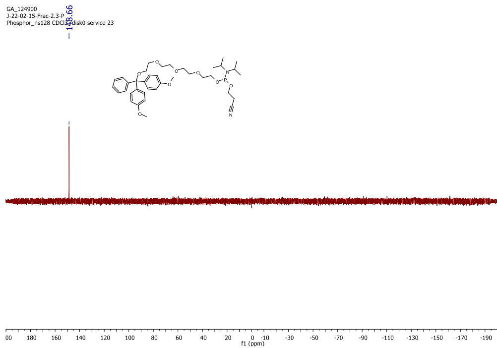
Figure 53. ^{31}\text{P} NMR of compound 3 in \text{CDCl}_3 .
