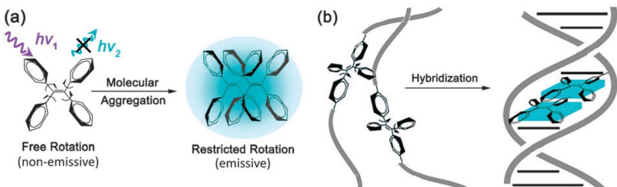
Figure 62. DATPE-modified DNA conjugates which exhibit AIE. Taken from [117] .
