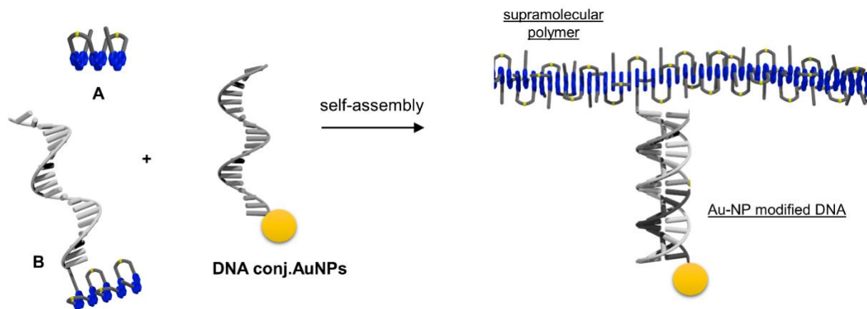
Figure 56. Illustration of the gold nanoparticles immobilization on the fibrillar supramolecular polymer.
