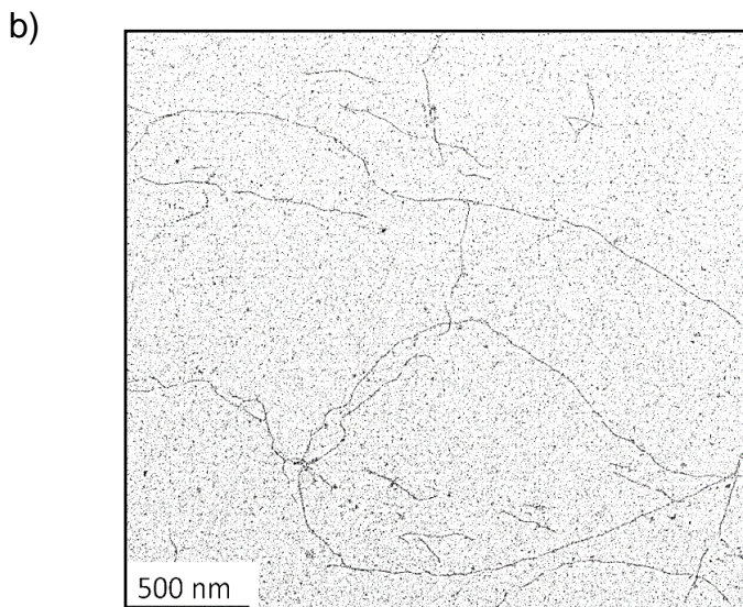
Figure 15. a) AFM analysis and b) TEM images of DNA-modified SPs. Sample for transmission electron microscopy (TEM) analysis was prepared according to the published procedure. [8] AFM of SPs modified with DNA strands were analysed on APTES-modified mica at 20 °C. Conditions: oligomer A, B, E, F (a); oligomer A, B (b).
