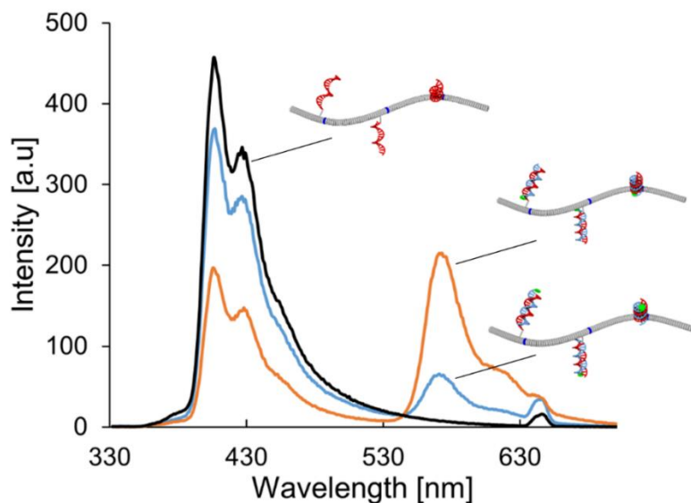
Figure 44. Fluorescence spectra of LHC6 (orange), LHC12 (blue) and self-assembled SPs (black) composed of oligomer A and N . Concentration of oligomers: A (0.5 \mu M) and 15 nM, N , H and O ; Conditions: 10 mM sodium phosphate buffer, pH 7.2, 120 mM NaCl, \lambda_{\text{ex}} : 322 nm.
