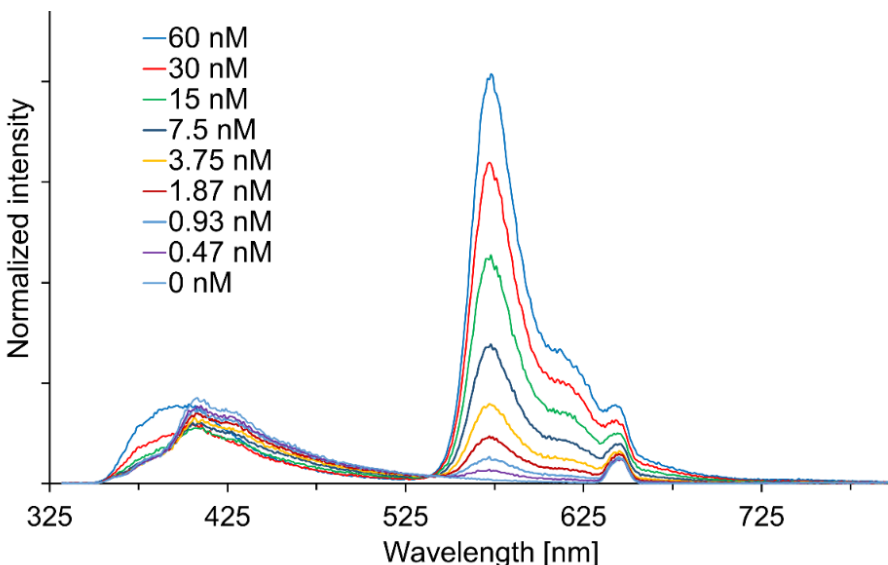
Figure 19. Emission spectra of oligomer A (0.5 \mu\text{M} ) in the presence of different concentrations of hybrid B*G after phenanthrene excitation (322 nm). Normalization was done by dividing the emission spectra by the absorption value of each individual sample at 322 nm.
