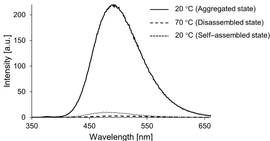
Figure 67. Fluorescence spectra of aggregated state: 20 °C (solid curve), disassembled state: 70 °C (dashed curve) and self-assembled: 20 °C (dotted curve); self-assembly was performed with slow cooling (1°C/min) from 70 °C to 20 °C. Conditions: oligomer 1 (1 \mu\text{M} ), 10 mM sodium phosphate buffer, pH 7.2, 20 vol% EtOH, \lambda_{\text{ex}} : 335 nm.
