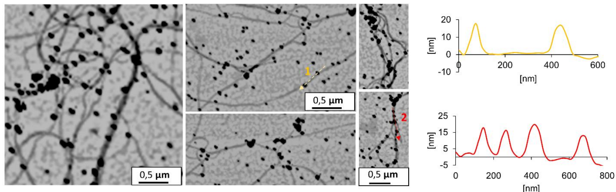
Figure 58. AFM images of the Au-NP modified DNA integrated into supramolecular polymer and the cross-sections profiles. Conditions: oligomer A (3 \mu\text{M} ), B (0.45 \mu\text{M} ), T (0.9 \mu\text{M} ) in 10 mM sodium phosphate buffer, pH 7.2, 120 mM NaCl.
