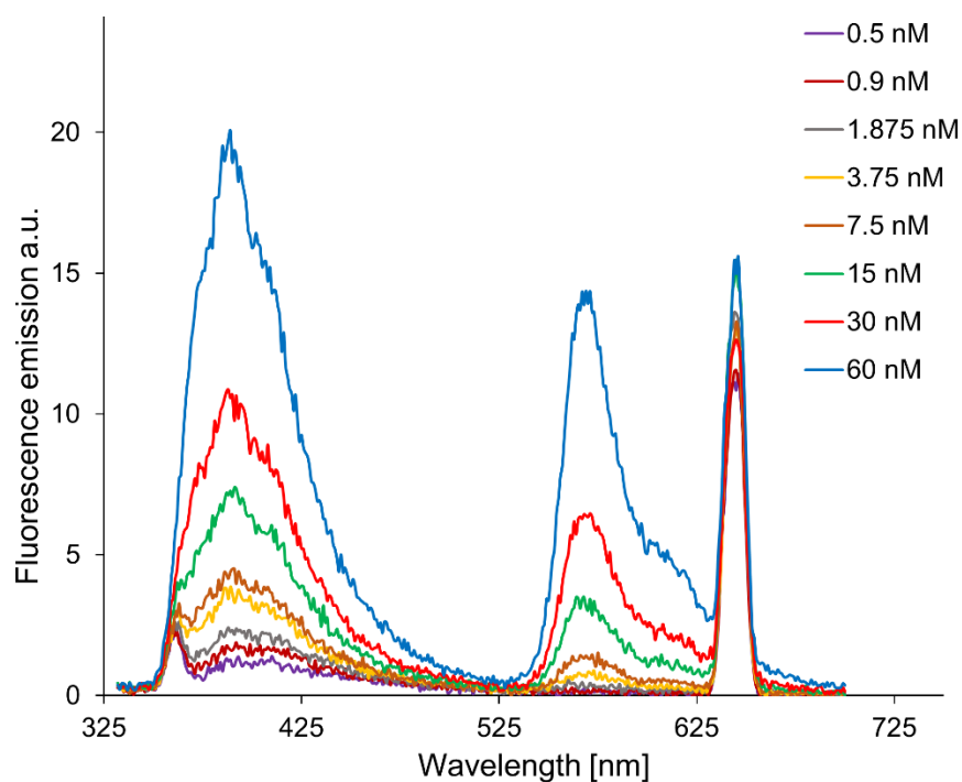
Figure 20. Emission spectra of different concentrations of hybrid B*G after excitation at 322 nm.
