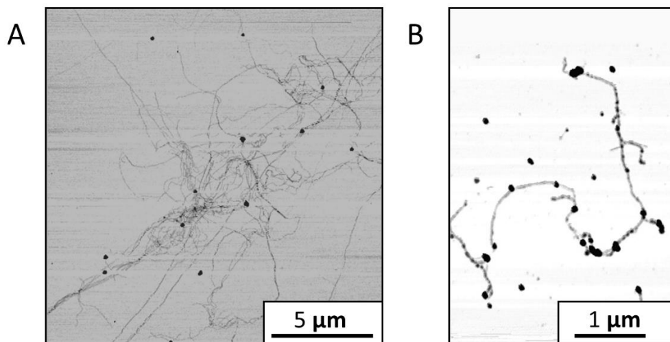
Figure 57. AFM images of the supramolecular polymers loaded with Au-NPs. Used concentrations for assembly of SPs; left: oligomer A (3 \mu\text{M} ), B (90 nM), T (150 nM); right: oligomer A (3 \mu\text{M} ), B (90 nM), and T (450 nM) in 10 mM sodium phosphate buffer, pH 7.2, 120 mM NaCl.
