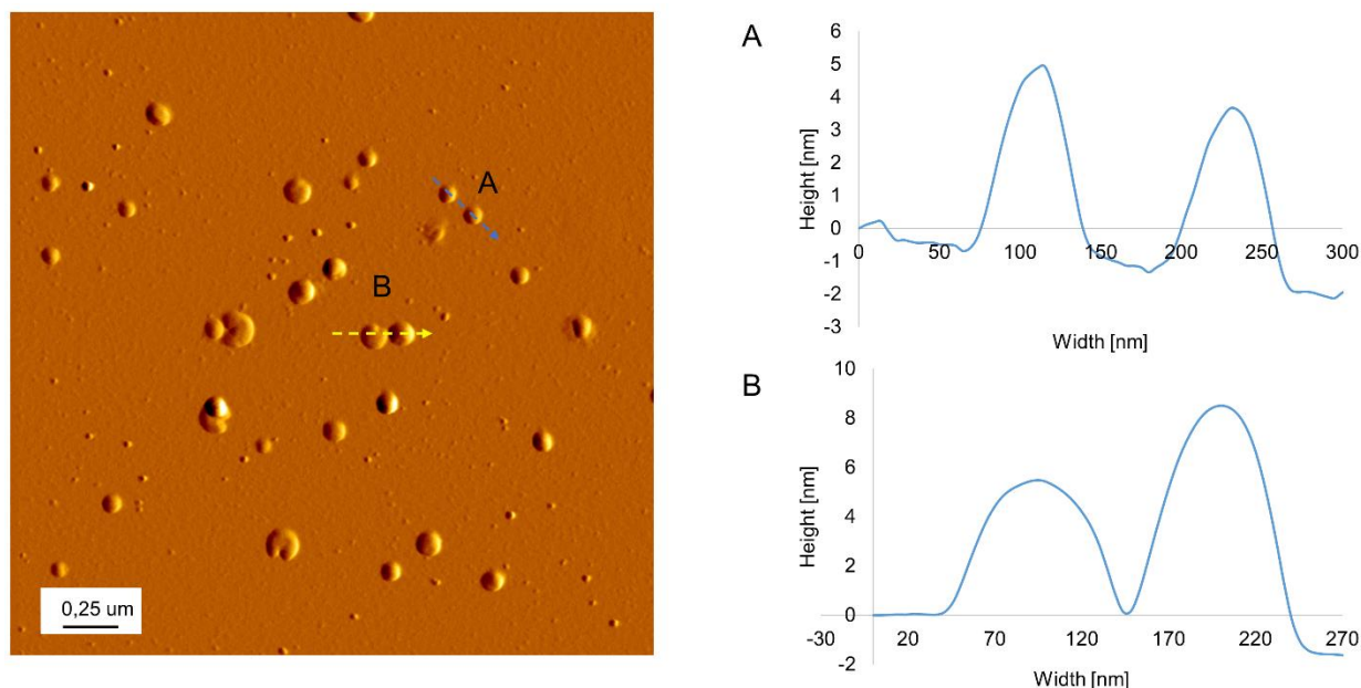
Figure 70. AFM images and cross-section profiles of the self-assembled oligomer 1 . Self-assembly was performed with slow cooling ( 1^\circ\text{C}/\text{min} ) from 70^\circ\text{C} to 20^\circ\text{C} . Conditions: oligomer 1 ( 10 \mu\text{M} ), 10 mM sodium phosphate buffer, pH 7.2, 20 vol% EtOH,
