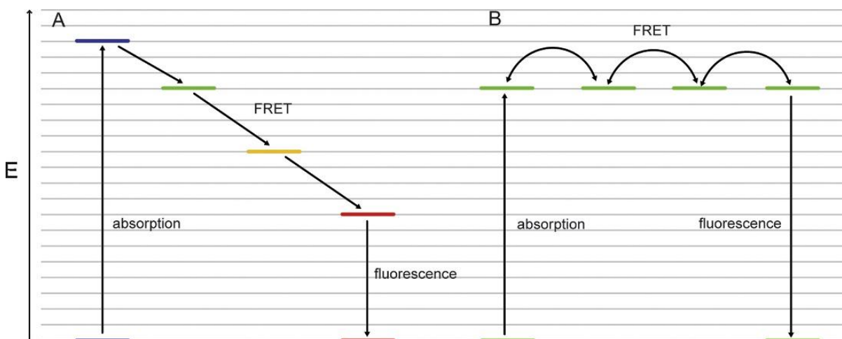
Figure 10. Schematic energy level diagram showing examples of multi-step hetero-FRET (A) and homo-FRET (B). Arrows indicate one of many potential energy pathways from the initial absorption at a donor fluorophore to the emission from the final acceptor. [42]
