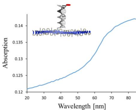
Figure 33. Melting curves of complexes: a) A and B ; b) A , B and H ( LHC1 ); c) B and H ; d) B , E and F ; e) I and H ; f) I , E and F ; g) I and E ; h) I and F ; i) A , B , C and D ( LHC3 ); j) A , B , C and F ( LHC2 ); k) A , B , D and E . Conditions: see Table 8.
