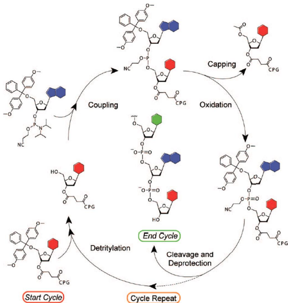
Figure 8. Typical cycle for the solid phase synthesis of oligonucleotides. [34]
