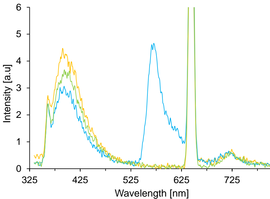
Figure 26. Fluorescence emission spectra of LHCs in the absence of oligomer A either lacking both Cy3 and Cy5 (green) or one of them (yellow and blue). Concentration of oligomers: 15 nM B , C , D , E and G ; Conditions: 10 mM sodium phosphate buffer, pH 7.2, 120 mM NaCl, \lambda_{\text{ex}} = 322 nm.
