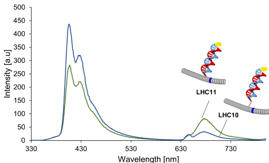
Figure 46. Fluorescence emission spectra of LHC10 (blue) and LHC11 (green). Conditions: concentration of oligomers: A (0.5 \mu\text{M} ), N, M, P (15 nM); 10 mM sodium phosphate buffer, pH 7.2, 120 mM NaCl.
