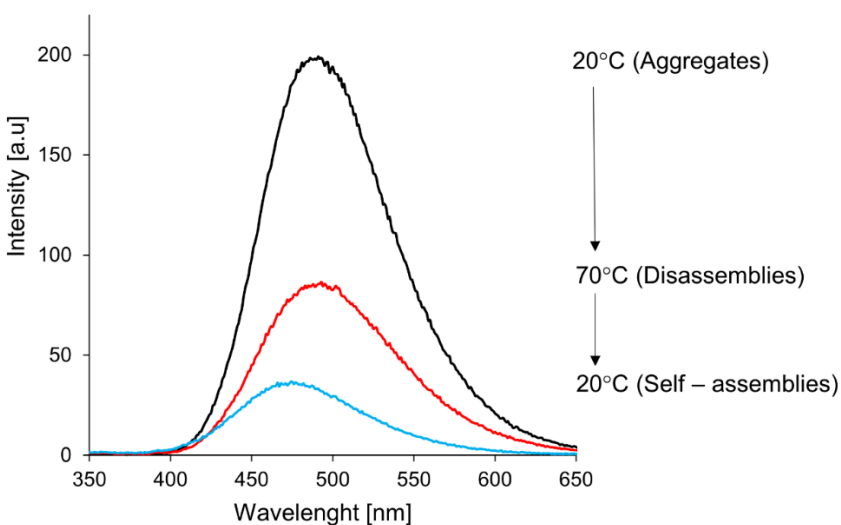
Figure 68. Fluorescence spectra of aggregated state: 20^\circ\text{C} (black curve), disassembled state: 70^\circ\text{C} (red) and self-assembled: 20^\circ\text{C} (blue); self-assembly was performed with cooling ( 1^\circ\text{C}/\text{min} ) from 70^\circ\text{C} to 20^\circ\text{C} . Conditions: oligomer 1 ( 10 \mu\text{M} ), 10 \text{ mM} sodium phosphate buffer, \text{pH } 7.2 , 20 \text{ vol}\% \text{ EtOH} , \lambda_{\text{ex}}: 335 \text{ nm} .
