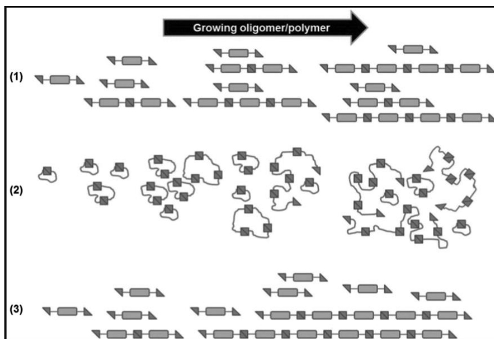
Figure 2. Three main mechanisms for the supramolecular polymer growth: (1) isodesmic, (2) ring-chain, (3) cooperative. [4]
