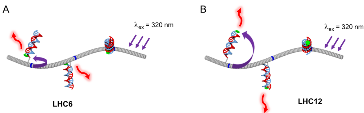
Figure 43. Illustration of the short-distance energy transfer in LHC6 (A) and long-distance energy transfer in LHC12 (B).
