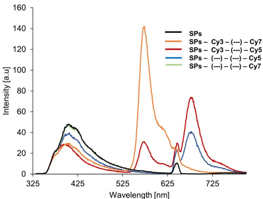
Figure 31. Additional fluorescence emission spectra for LHCs missing the first or the intermediate donor-acceptor. Concentration of oligomers: A (0.5 \mu M) and B, E, G, P, R, S (15 nM). Conditions: 10 mM sodium phosphate buffer, pH 7.2, 120 mM NaCl, \lambda_{\text{ex}} = 322 nm.
