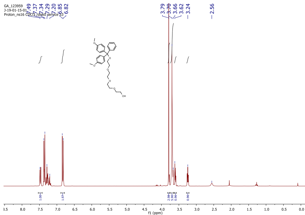
Figure 51. ^1\text{H} NMR of compound 2 in \text{CDCl}_3 .
