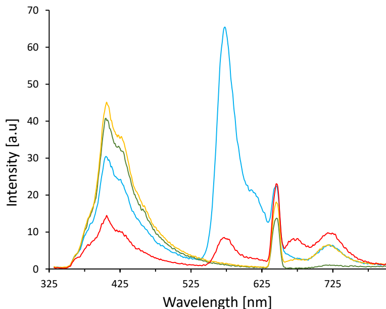
Figure 25. Fluorescence emission spectra of LHCs either lacking both Cy3 and Cy5 (green) or one of them (yellow and blue) compared to LHC3 (red). Concentration of oligomers: A (0.5 \mu\text{M} ), 15 nM B, C, D, E, and G ; Conditions: 10 mM sodium phosphate buffer, pH 7.2, 120 mM NaCl, \lambda_{\text{ex}} = 322 nm.
