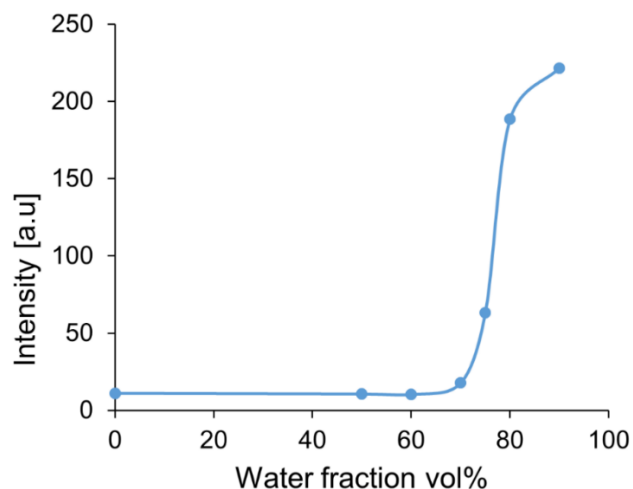
Figure 65. Changes in the fluorescence intensity of oligomer 1 with variation of the water / EtOH ratio. Concentration of oligomer 1 : 1 \mu M, 10mM sodium phosphate buffer pH 7.2, \lambda_{ex} : 335 nm.
