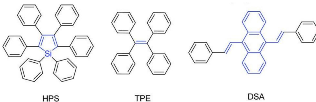
Figure 60. Examples of typical AIEgens. Taken from [110] .
