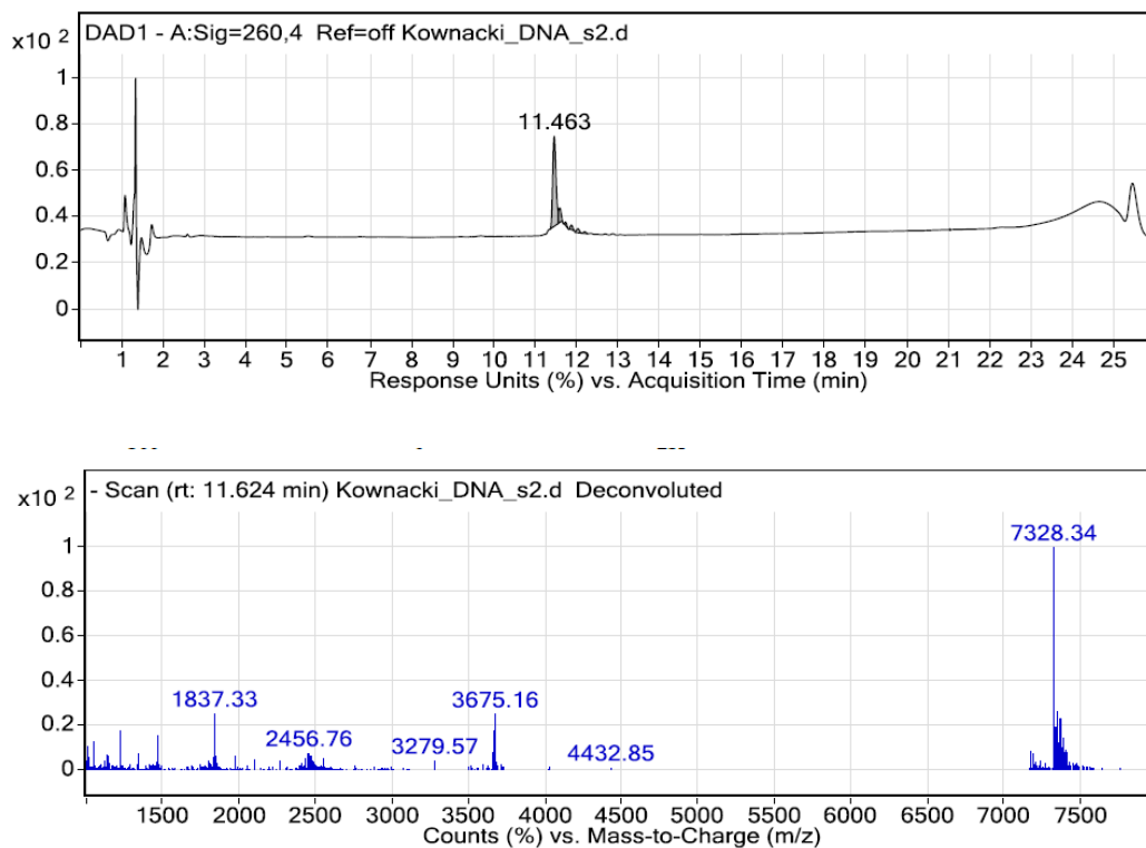
Figure 29. LC-MS analysis of oligomer K.
