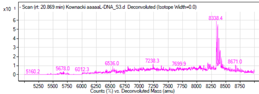
Figure 47. MS analysis of oligomer L.
