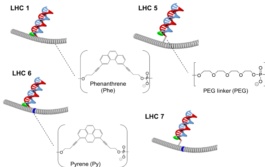
Figure 34. Illustrations of different LHCs: pyrene (dark blue), phenanthrene (grey), PEG linker (grey bar), Cy3 (green).
