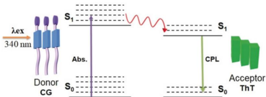
Figure 11. Illustration of the energy level diagram for ET-associated CPL mechanism. [41]
