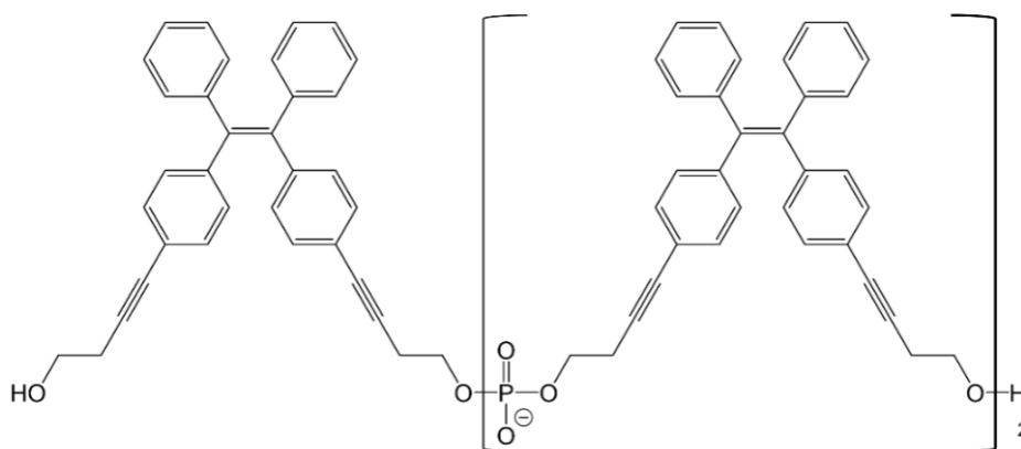
Figure 63. The phosphodiester-linked Z-DATPE trimer ( 1 ).
