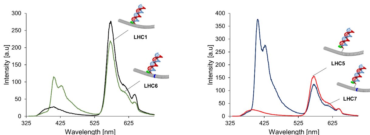
Figure 41. Fluorescence emission spectra. Left: LHC1 (black) and LHC6 (green). Right: LHC5 (red) and LHC7 (blue). Concentration of oligomers: A (0.5 \mu\text{M} ), B, L, M, N, H (15 nM); Conditions: 10 mM sodium phosphate buffer, pH 7.2, 120 mM NaCl, \lambda_{\text{exc.}} : 322 nm.
