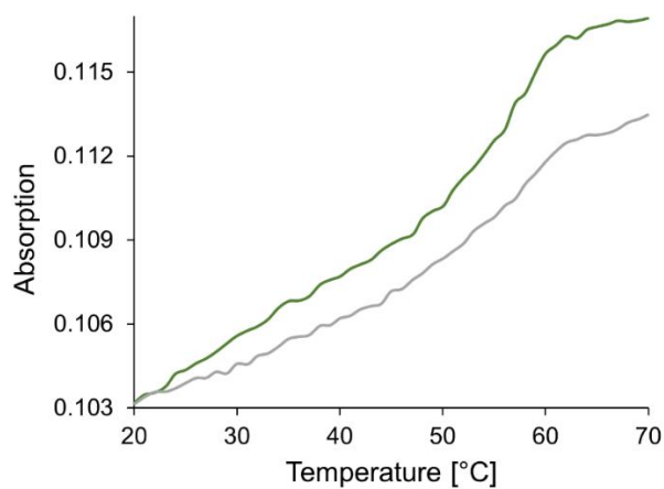
Figure 72. Heating-cooling curve of oligomer 1. Ramp 1: cooling (green), ramp 2: heating (gray). Concentration of oligomer 1: 1 \mu M, 10mM sodium phosphate buffer pH 7.2, \lambda_{ex.} : 335 nm. Temperature gradient: 0,3 ^{\circ} C/min. Absorbance was recorded at 250 nm
