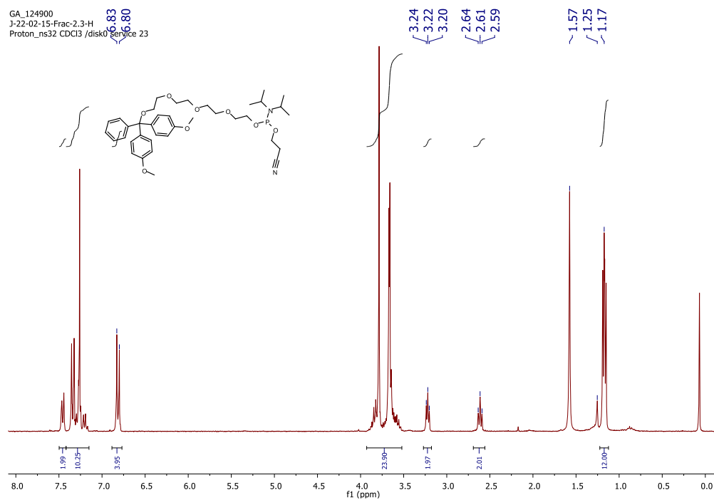
Figure 52. ^1\text{H} NMR of compound 3 in \text{CDCl}_3 .
